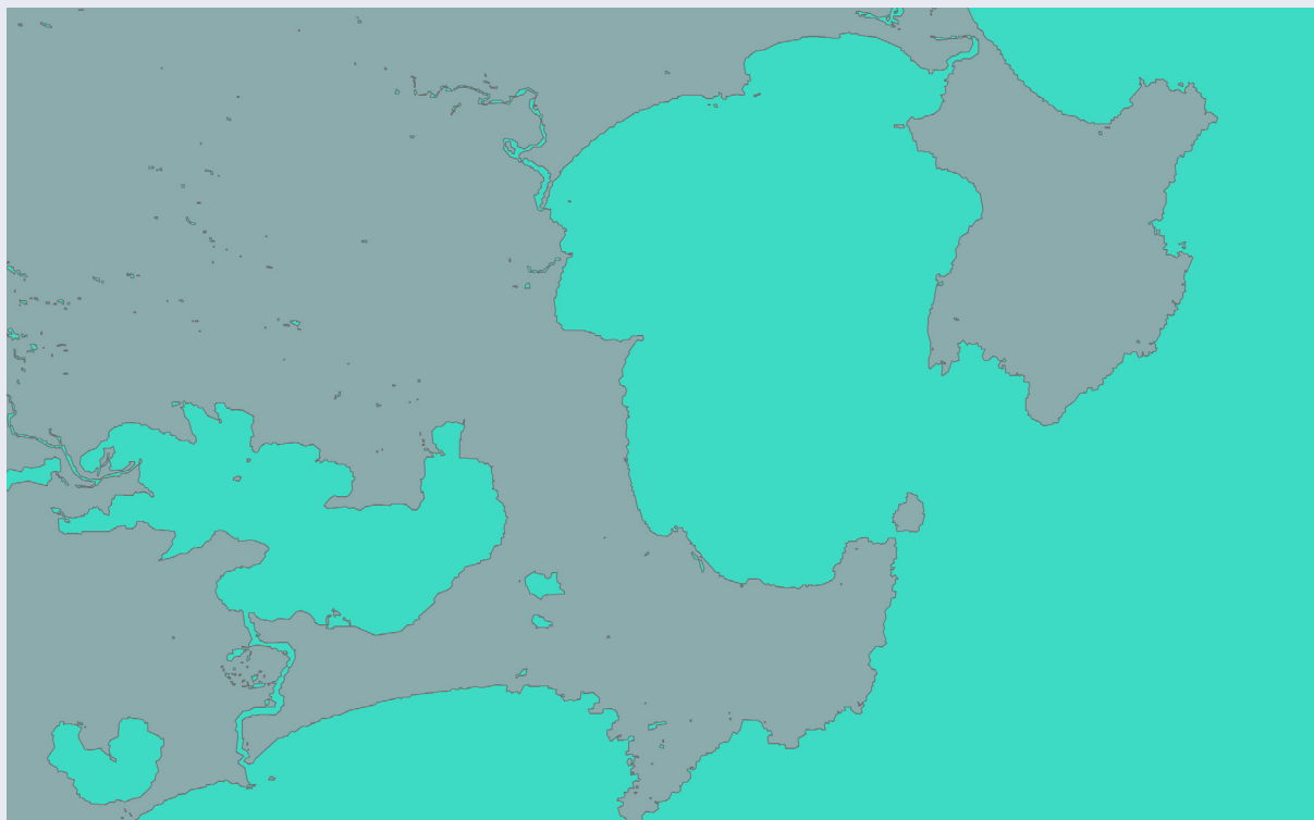
Figure 10.10 Secondary segmentation
