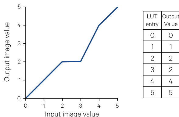
Figure 4.16 LUT operations for rescaling image data values
